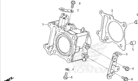
E-6 CYLINDER
