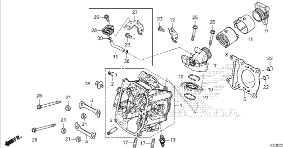
E-6 CYLINDER
