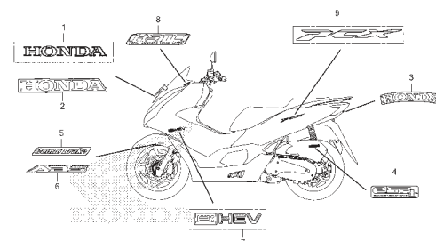
F-48 MARK/EMBLEM
