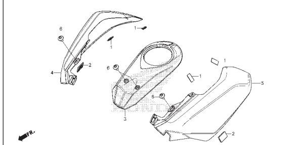
F-16 TANK COVER
