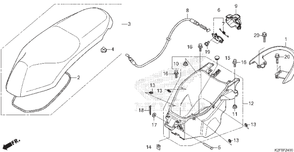
F-24 SEAT/LUGGAGE BOX
