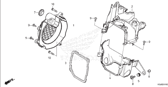
E-1 SHROUD/FAN COVER
