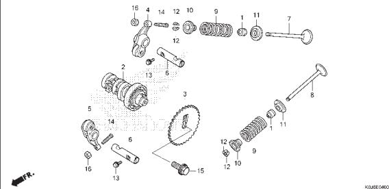
E-4 CAMSHAFT/VALVE
